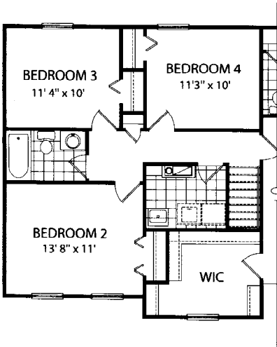
Second Floor Plan Somerset B
